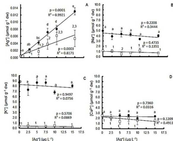
FIGURE 2. Metal levels [ \mu\text{mol metal g}^{-1} dry weight for embryo ( \pm SE)]. Live embryos have the circle symbol, while dead embryos have the square symbol. Zebrafish embryos at 24 hpf relative to the nominal total Ag exposure concentrations. Measured silver (A), sodium (B), potassium (C), and calcium (D) concentrations were assessed in embryos exposed to \text{AgNO}_3 . Each exposure condition had six independent repeats, and each one contained 170 embryos at the beginning of the exposure. The total number of embryos analysed for each condition was (20). Different letters and numbers refer to statistical differences between concentrations (ANOVA, p < 0.05 ). Similar letters and numbers represent non-statistically significant differences between concentrations (ANOVA, p > 0.05 )
