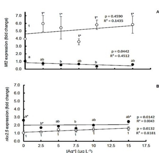
FIGURE 5. Relation to silver concentrations: (A) the expression of mt2 ; (B) nkx2.5 . Solid circle embryos were sampled at 24 hpf, open circle embryos were sampled at 72 hpf. The 2^{-\Delta\Delta Ct} technique was utilized to calculate fold changes in gene expression, using \beta -actin as a housekeeping gene. Each treatment has three samples, and the data are means \pm S.E.M . ANOVA under p < 0.05 shows that there is a significant effect between the concentrations when different letters appear. A non-considerable impact ( p > 0.05 ) is indicated by the same numbers. * Explains how 24- and 72-hour-aged embryos differ from one another
