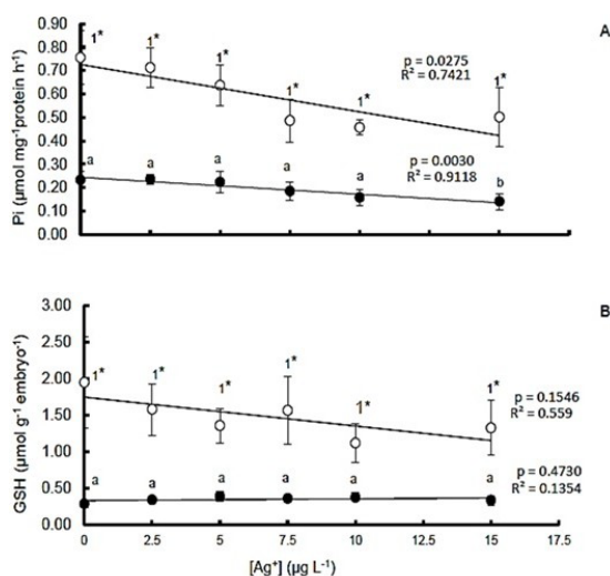
FIGURE 4. Average Na^+ K^+-ATPase (A), GSH (B) in living embryos at 24h and 72 hours post-exposure to silver (solid and open circles, respectively). Each replication has 170 embryos, and the results are means \pm SE ( n=6 ). However, the ANOVA table test revealed that Ag had no statistically significant influence on total GSH levels or Na^+ K^+-ATPase activity ( p > 0.05 ). LSD significantly affected Na^+ K^+-ATPase at 10 \mu g/L^{-1} versus control. *Mean that embryos aged 24 and 72 hours differ significantly ( p < 0.05 )
